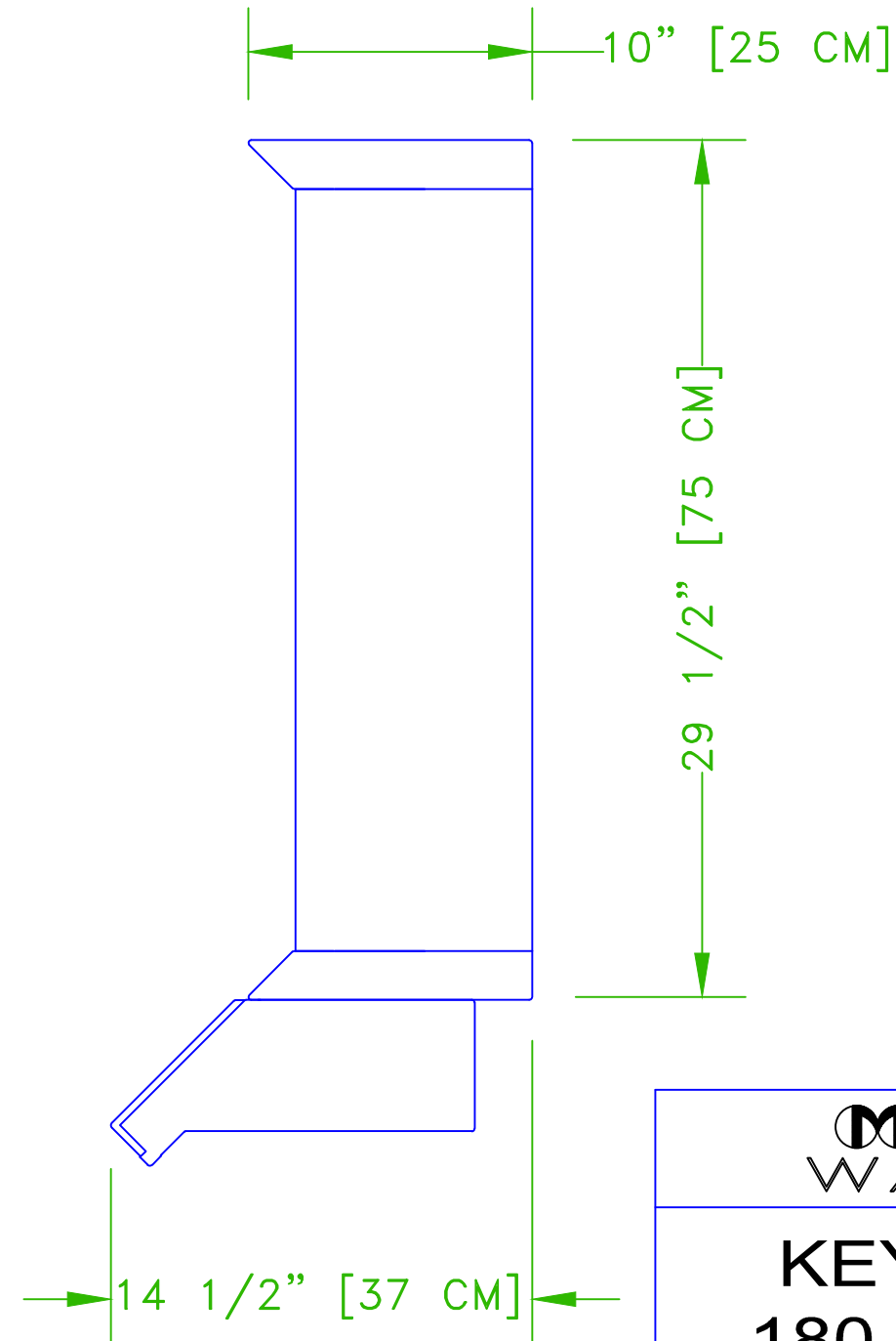
SIDE VIEW
